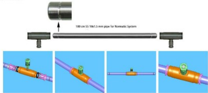
NORMATIC PUSH IN FITTING SYSTEM
